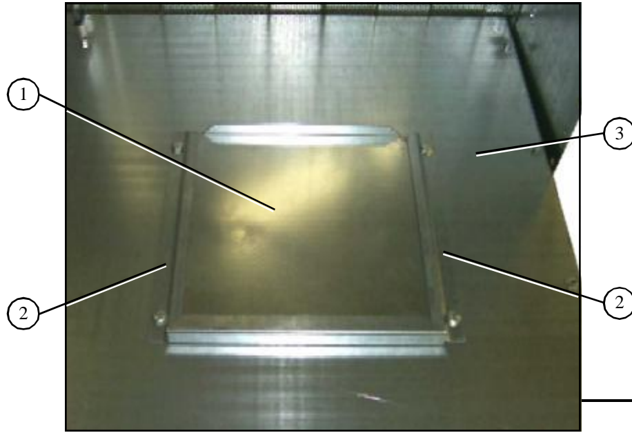
Plenum divider floor sections.
